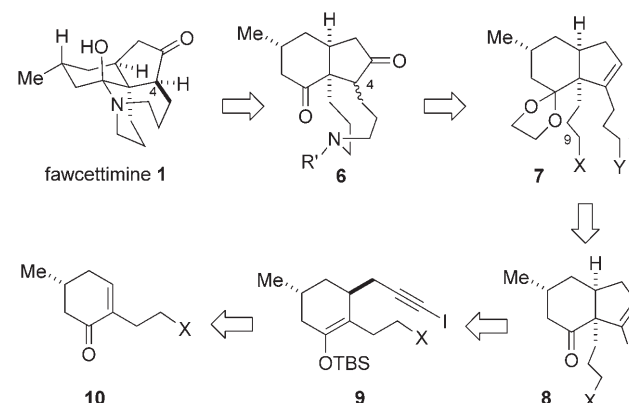
Scheme 1. Retrosynthetic analysis of 1 . TBS = tert -butyldimethylsilyl.
