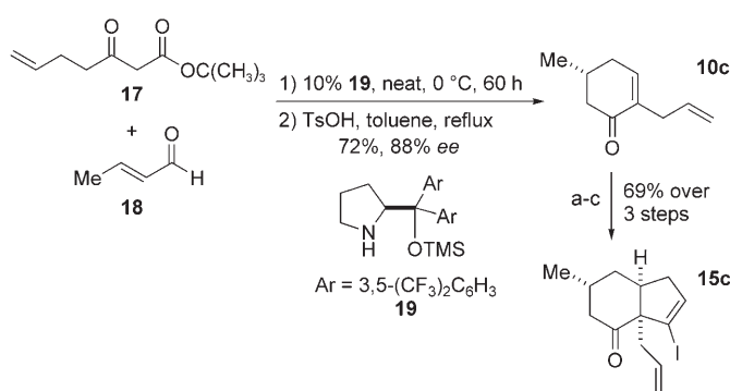
Scheme 3. Organocatalytic/gold-catalyzed cyclization approach to the hydridanone core of 1 . a) 12 , TBSOTf, CH 2 Cl 2 , -78 °C; b) NIS, AgNO 3 , DMF, 0 °C; c) 10% [Ph 3 PAu]Cl, 10% AgBF 4 , CH 2 Cl 2 /MeOH 10:1, 40 °C. Ts = p -toluenesulfonyl.
