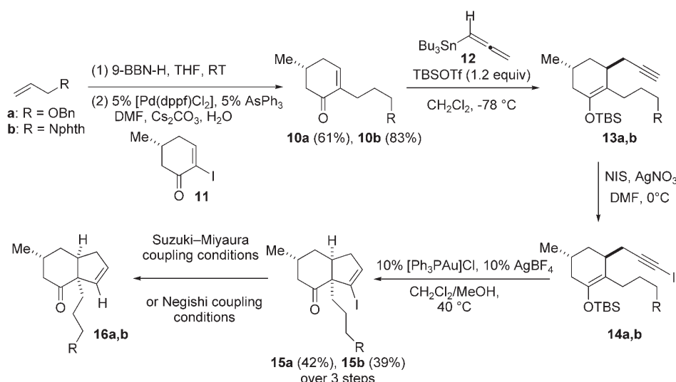
Scheme 2. Cross-coupling route to the hydridanone core of 1 . phth = phthaloyl; dppf = 1,1'-bis(diphenylphosphino)ferrocene, 9-BBN-H = 9-borabicyclononane, DMF = dimethylformamide.
